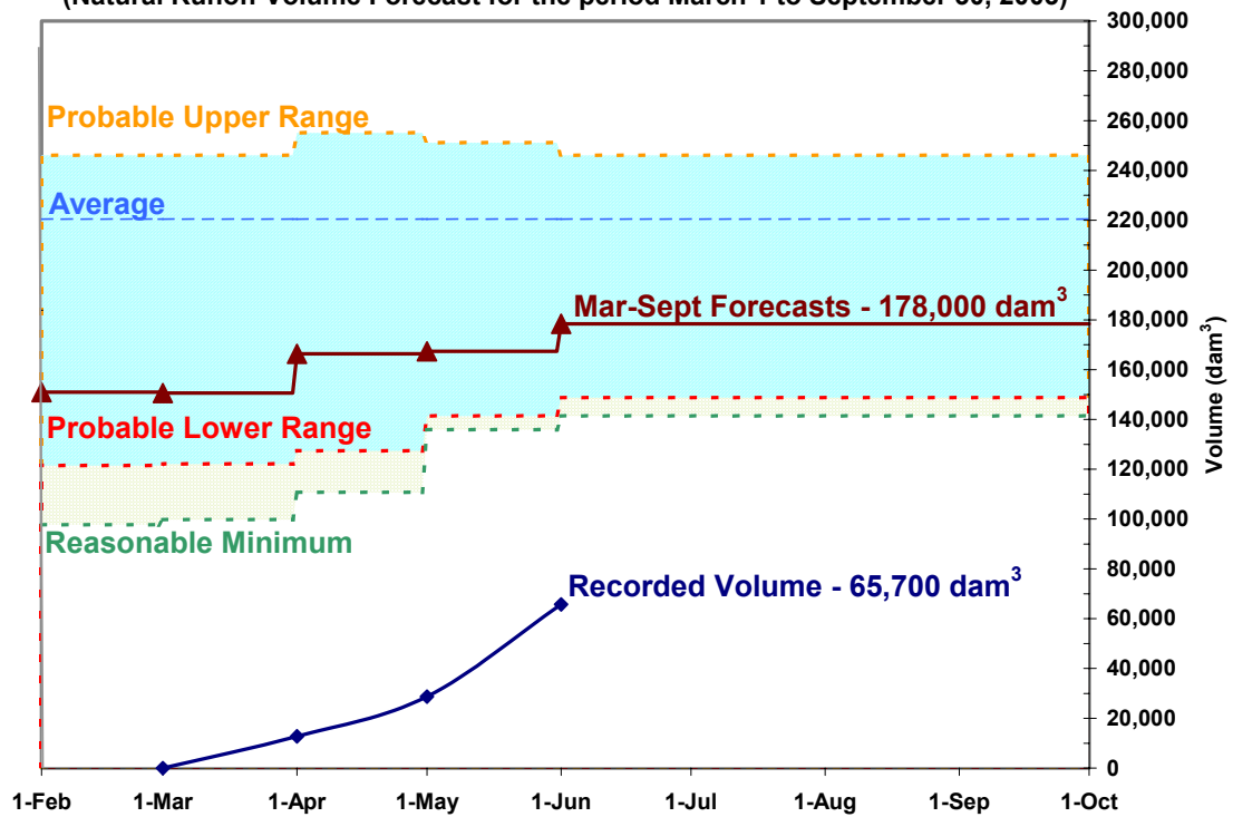
Water Supply Forecast as of June 1, 2003 for the Elbow River at Bragg Creek (Natural Runoff Volume Forecast for the period March 1 to September 30, 2003)
