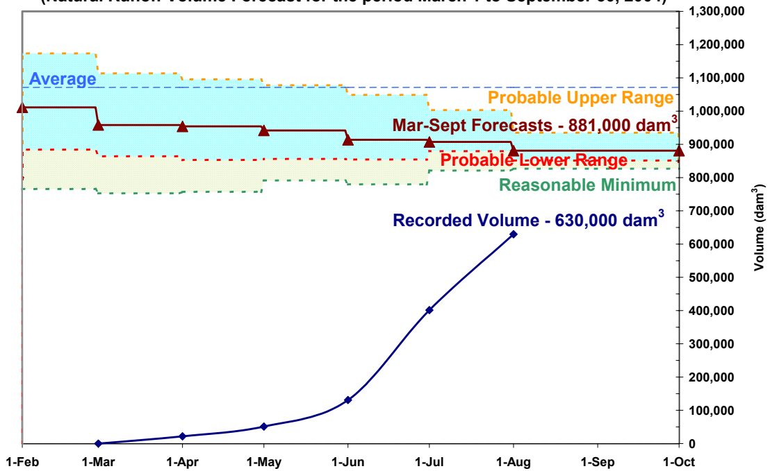
Water Supply Forecast as of August 1, 2004 for the Bow River at Banff (Natural Runoff Volume Forecast for the period March 1 to September 30, 2004)
