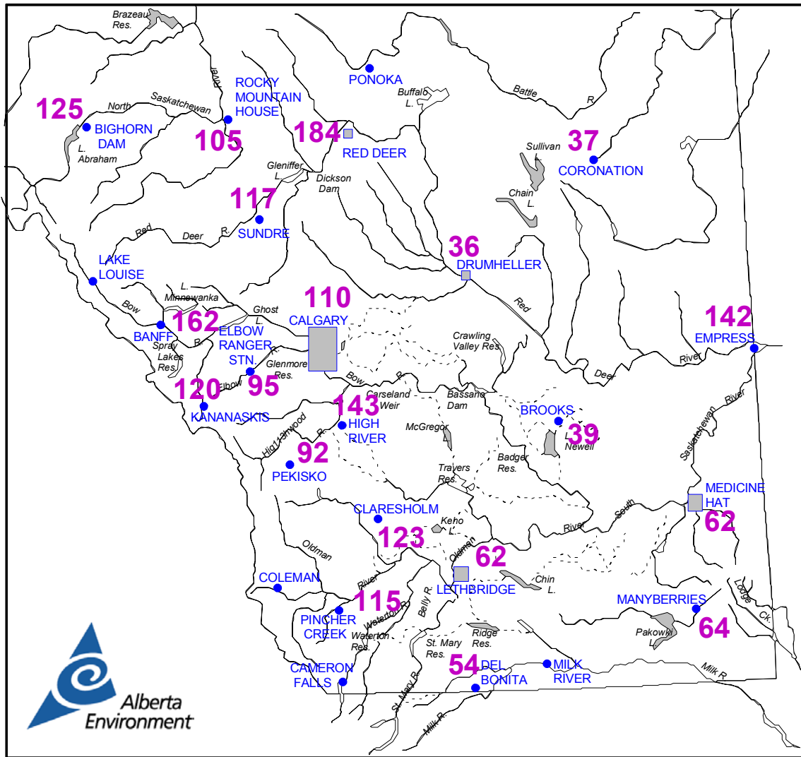
Figure 2 Precipitation Southern Alberta March 1 to 31, 2003 as a percent of Normal Normal = 100% (based on 1961 to 1990 data)
